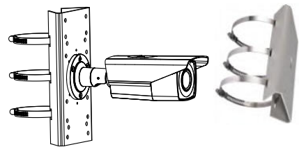
P-275ZJ Pole mount
