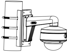
P-275ZJ Vertical Pole Mount
