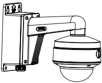
P-273ZJ-140B Wall Mount
